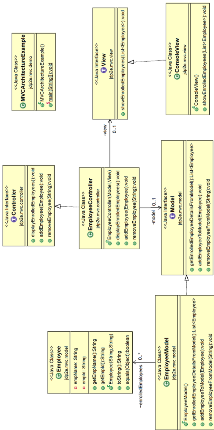
Figure 26-6. Class diagram
