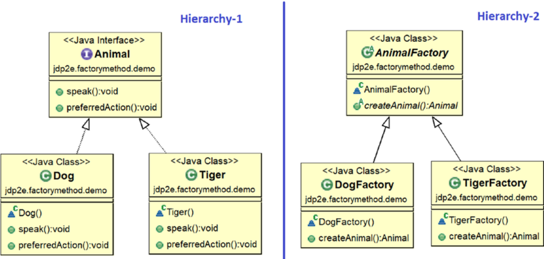
Figure 4-3. The two class hierarchies in our example
