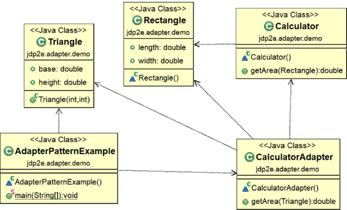
Figure 8-3. Class diagram
