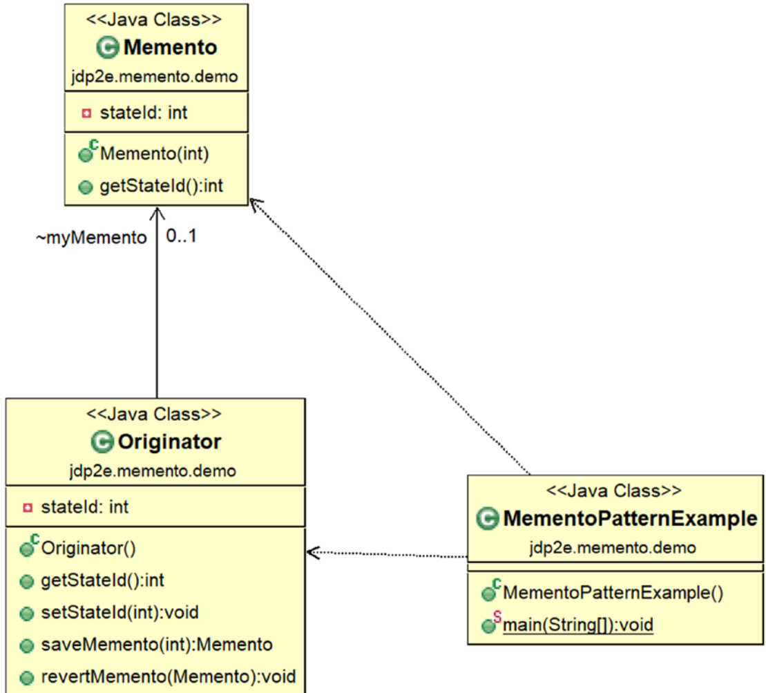
Figure 19-1. Class diagram
