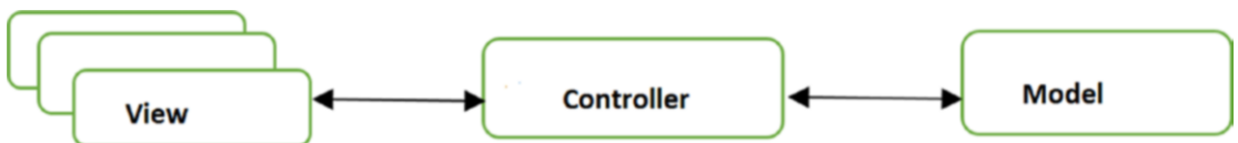
Figure 26-3. A MVC framework with multiple views
