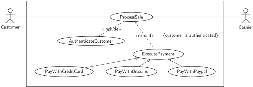
Fig. 4.13 Use cases of CoCoME payment possibilities
