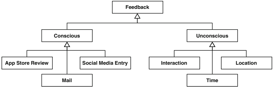
Fig. 5.2 A taxonomy of feedback provided by the end users of a mobile application
