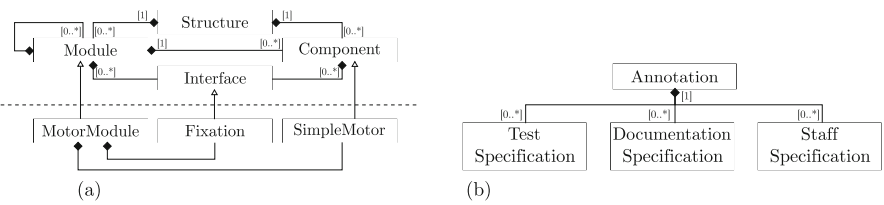
Fig. 10.23 aPS meta-models. (a) Structural aPS meta-model. (b) Non-structural aPS annotation meta-model [Hei+18a]
