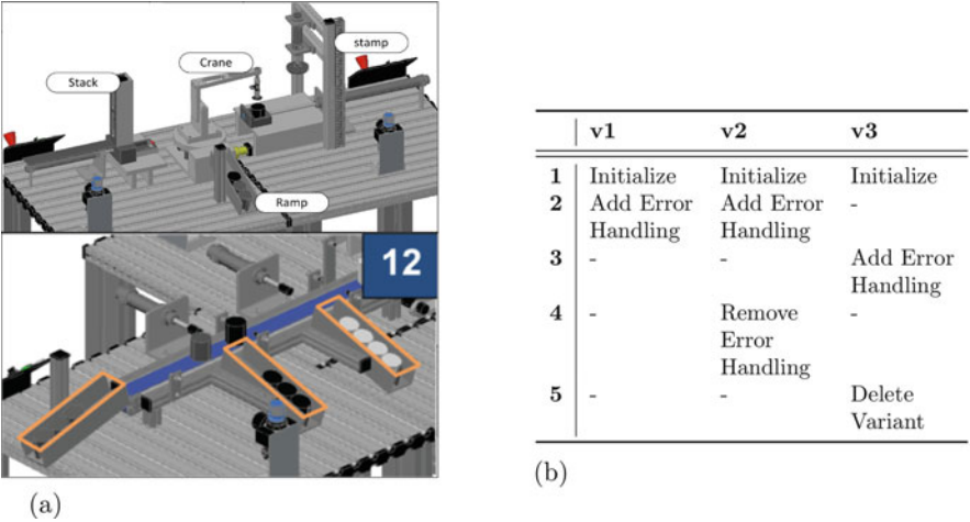
Fig. 7.1 (a) xPPU evolution scenario. (b) Overview of xPPU evolution steps
