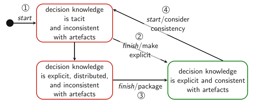
Fig. 6.12 State diagram of decision knowledge and artefacts. The state on the lower right side is the preferred state
