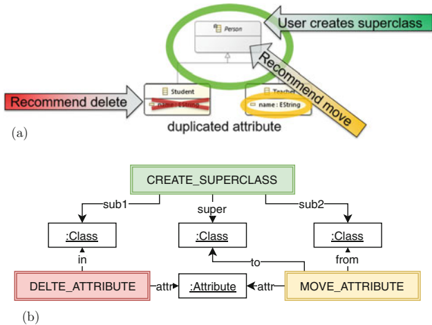
Fig. 10.15 Example of Pull-up-Attribute recommendation and blueprint. (a) Example Pull-up-Attribute recommendation (red and yellow) after a user creates a superclass (green). (b) Example blueprint for recommendation in a
