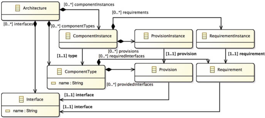
Fig. 9.11 The core of the IAL
