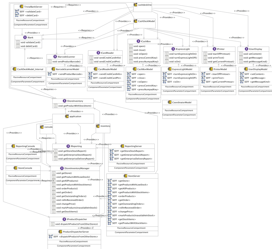
Fig. 12.5 The CoCoME architecture in an PCM system diagram, as extracted with Coding
