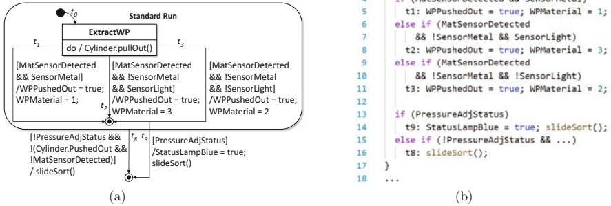
Fig. 7.2 Extract from an xPPU variant. (a) Test model. (b) Code
