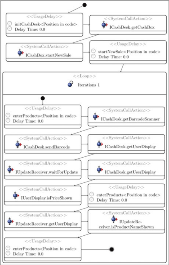
Fig. 12.8 Use Model of the ProcessSale use case extracted from unit tests [Lan+16]
