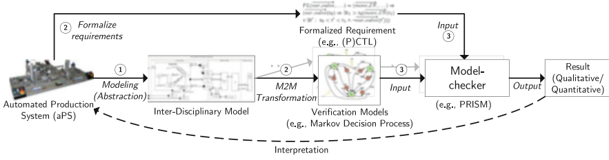
Fig. 11.3 MoDEMMiCAS approach for model-checking interdisciplinary systems (simplified)
