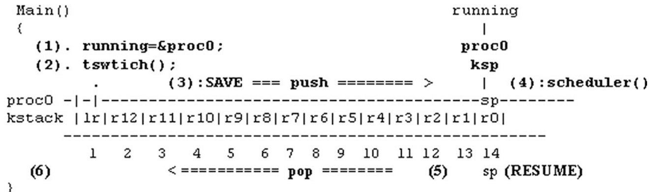
Fig. 5.1 Execution diagram of proc0
