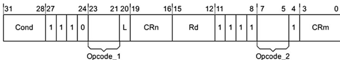
Fig. 6.2 MCR and MRC instruction format
