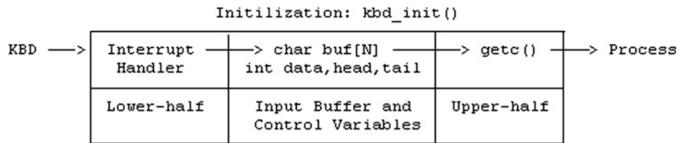
Fig. 3.5 KBD driver organization
