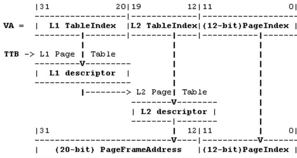
Fig. 6.6 Translation of Small Pages
