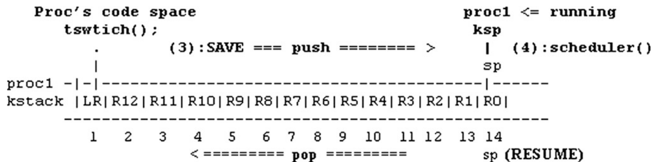
Fig. 5.2 Execution diagram of proc1
