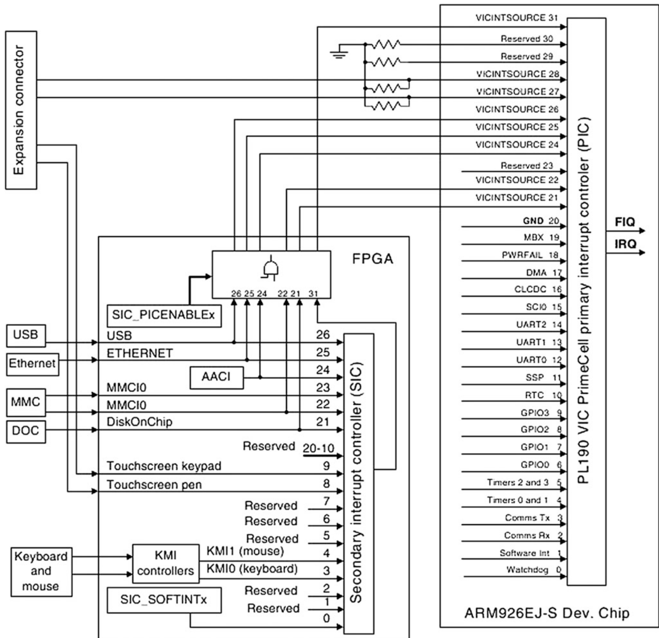
Fig. 3.2 VICs in ARM926EJ-S Board
