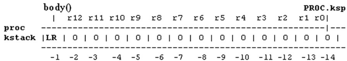
Fig. 5.4 Initial stack contents of process
