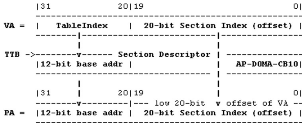
Fig. 6.4 Translation of Section References
